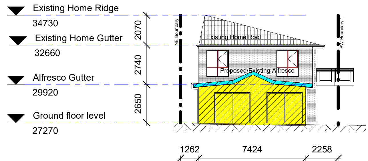
3 A9 North West Elevation np 1 : 150
